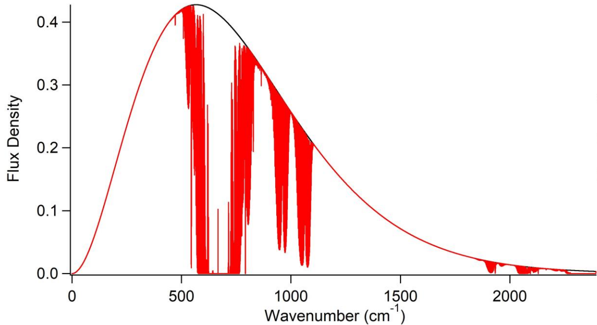
Planck Distribution times Transmittance
