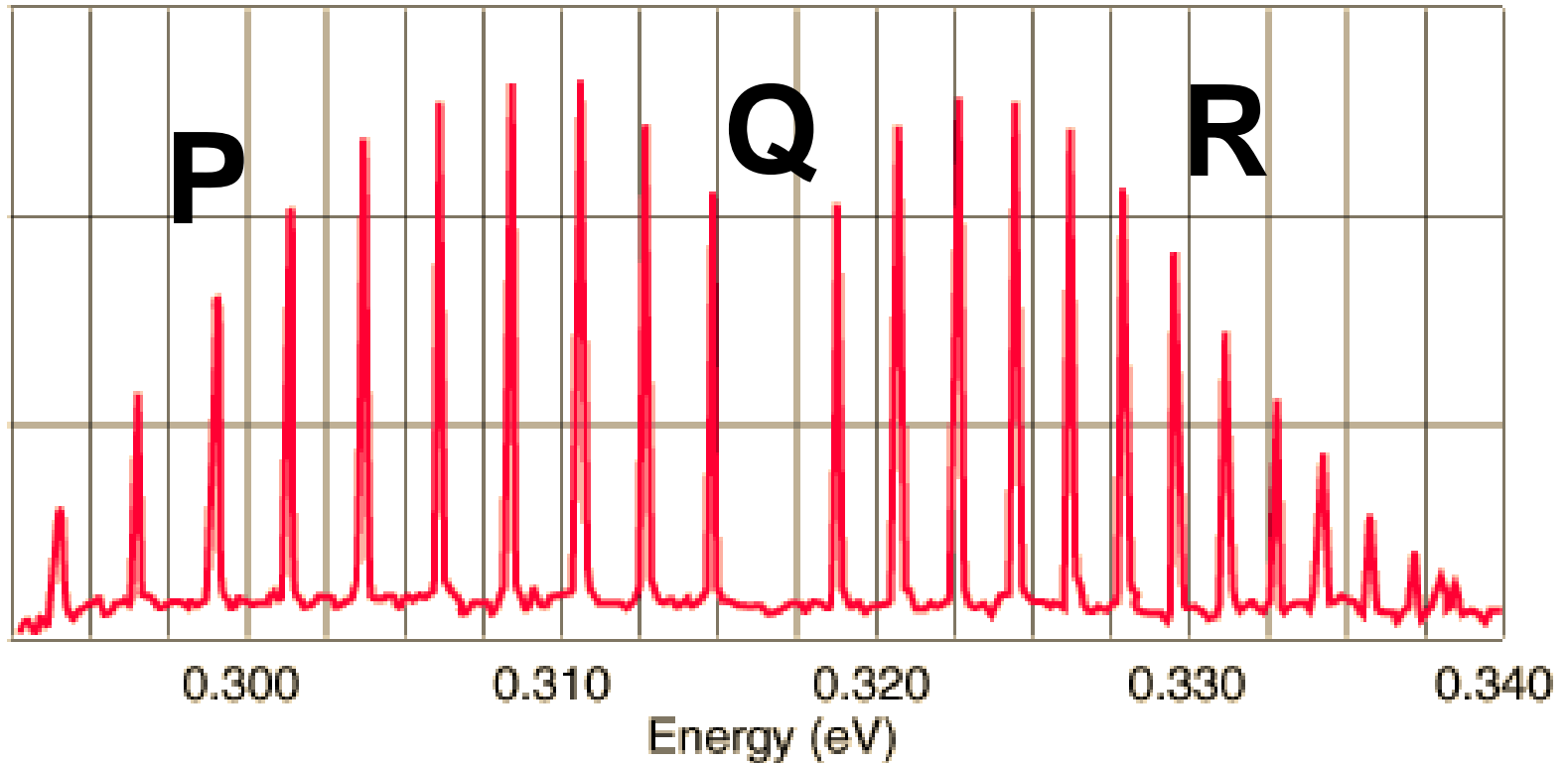
Sketch of the vibration-rotation spectrum of HBr
